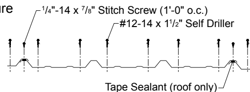
PBR-Panel Fastening Pattern
