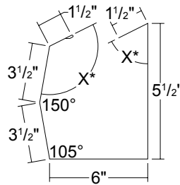
Lengths 10'-2" and 20'-3" *Specify Slope Angle
