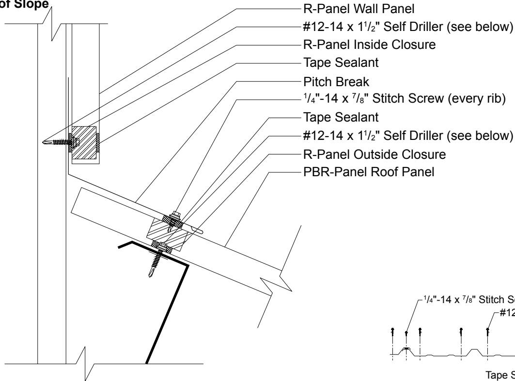
PBR-Panel Fastening Pattern
