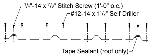
PBR-Panel Fastening Pattern
